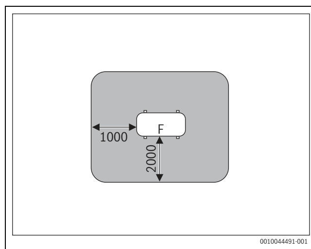
Fig. 17 Protection zone for installation on the floor, on the site or roof - dimensions in mm
