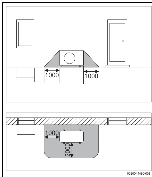
Fig. 16 Protection zone, floor-standing outdoor unit against a wall - dimensions in mm
