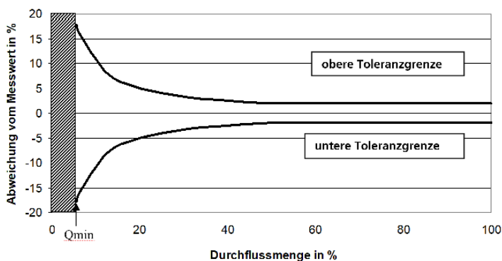
Toleranzgrenzen Figur 138 4G/6G, DN 15 – DN 50
