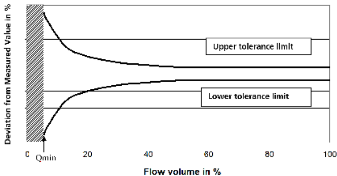
Tolerance Limits Figure 138 4G/6G, DN 15 – DN 50
