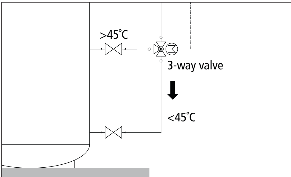
Figure 1 - Schematic diagram of the 3-way valve.
